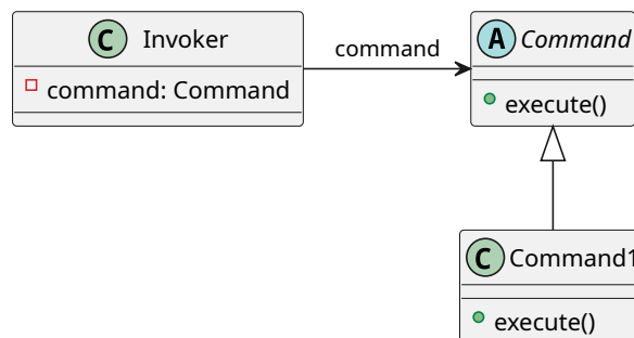
Figure 318: UML diagram for the Command Pattern
